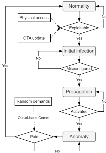
Fig. 1. Threat model lifecycle against the device
