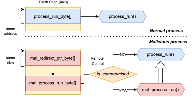
Fig. 4. Malicious function copy in flash
