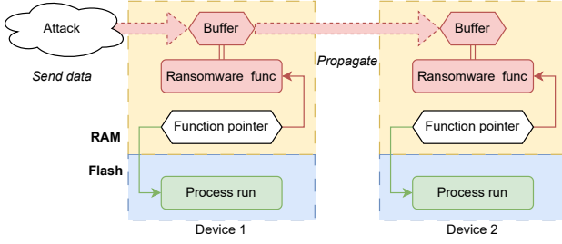
Fig. 3. Malicious function copy in RAM
