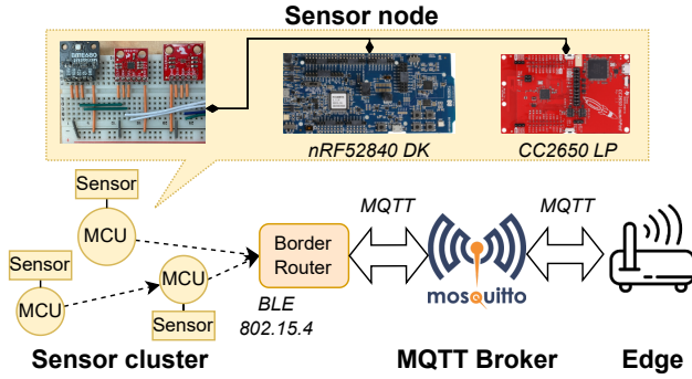
Fig. 2. Sensing network architecture
